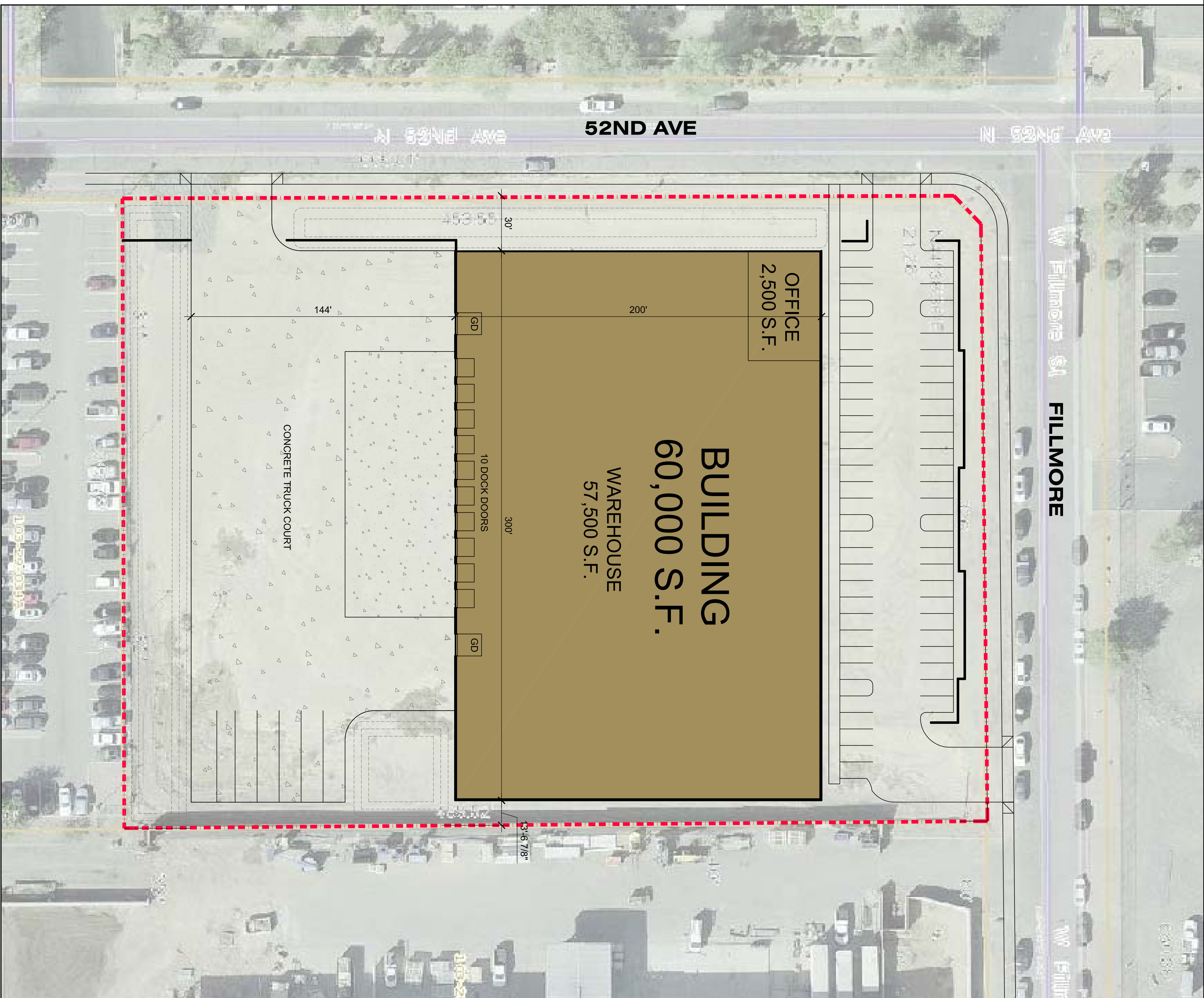
CONCEPTUAL SITE PLAN SCALE: 1"=30'-0" GRAPHIC SCALE
